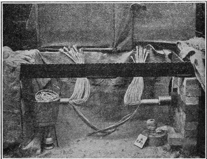
Fig. 7.—CABLE ENDS CUT IN READINESS FOR JOINTING.
