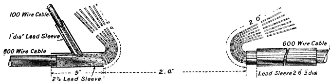
C - Arrangements for Teed or Y Joint.
