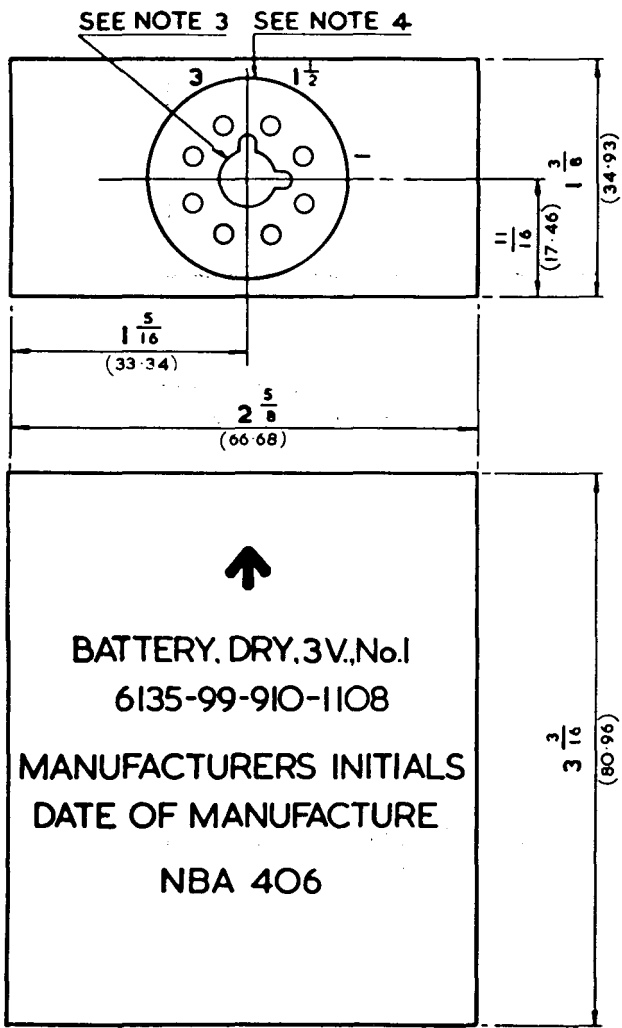
THIRD ANGLE PROJECTION
